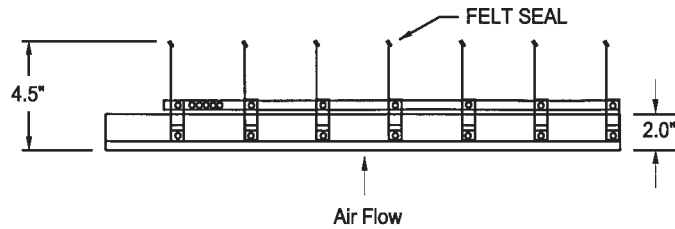
SECTION (OPEN)
